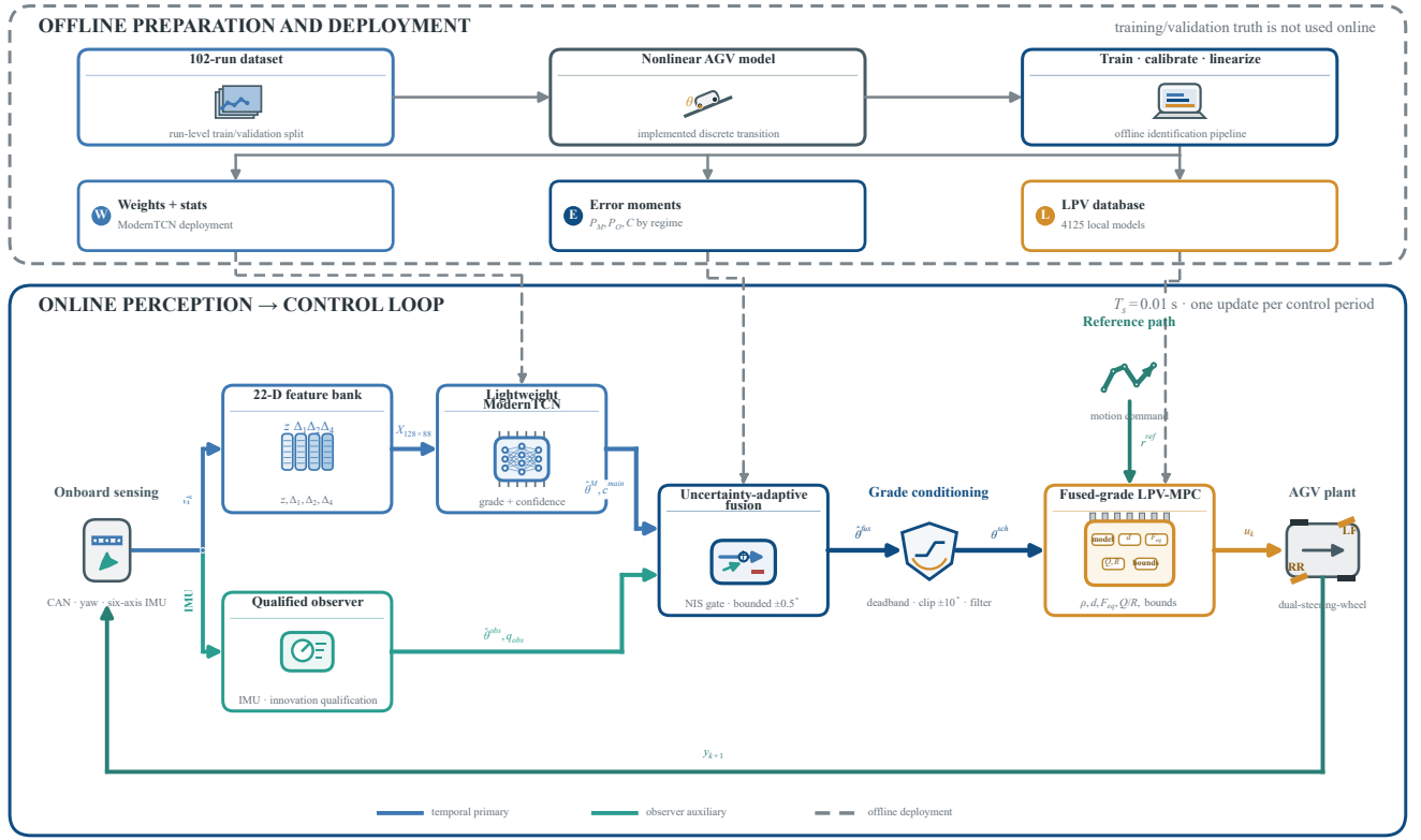
FIGURE 2. Overall slope-aware perception-and-control framework. The online loop separates the history-based primary branch from the bias-compensated six-axis Qualified observer branch. ModernTCN-delta supplies the primary grade and confidence; the Qualified observer contributes only an innovation-qualified, bounded correction with exact fallback to the ModernTCN estimate. The conditioned grade \hat{\theta}_k^{\text{sch}} synchronously updates the LPV scheduling vector, measured-disturbance channel, grade feedforward, weights, and constraints before the constrained MPC command is applied to the nonlinear AGV plant. Dashed gray arrows denote offline deployment of normalization statistics and network weights, fusion error moments, and the 4125-model LPV database.
