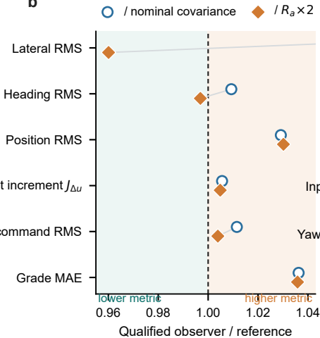
Covariance sensitivity: R_a \times 2 , Q_g \times 0.5
