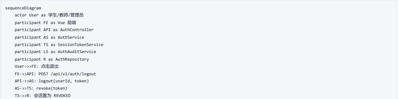
图 5-4 SC-AUTH-03 退出登录组件级顺序图
