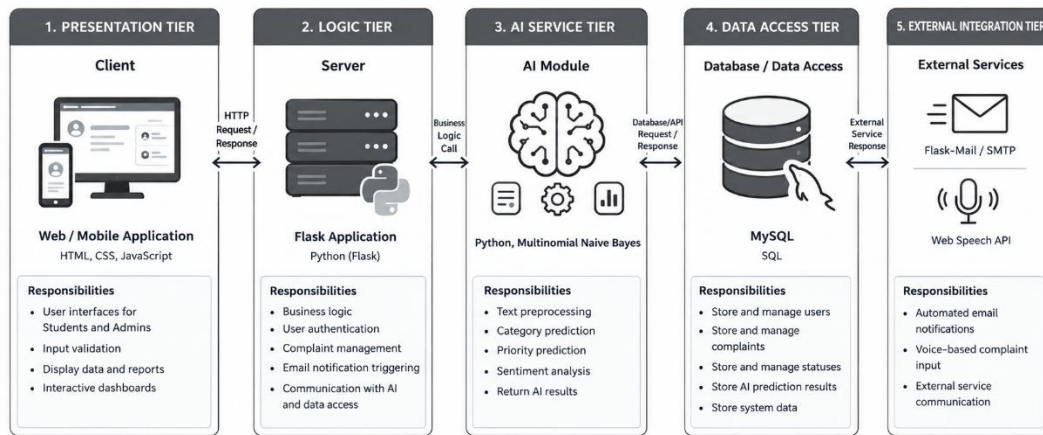
Figure 5.1: System Architecture
