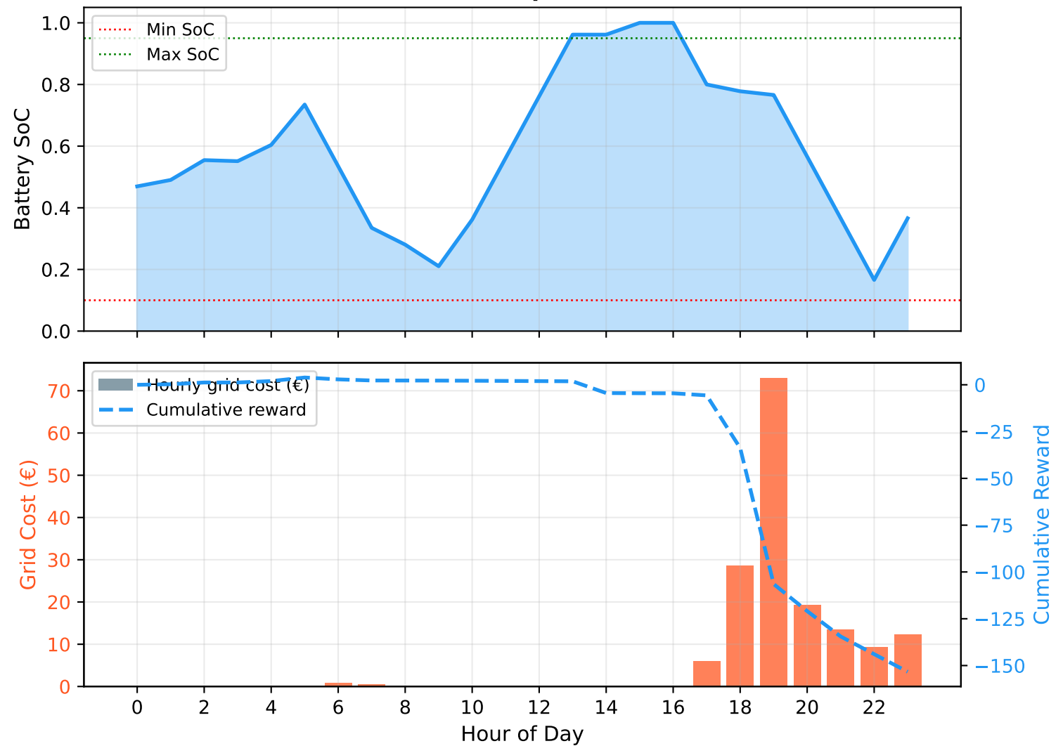
Station 1: 24-Hour Dispatch (Solar + BESS)
