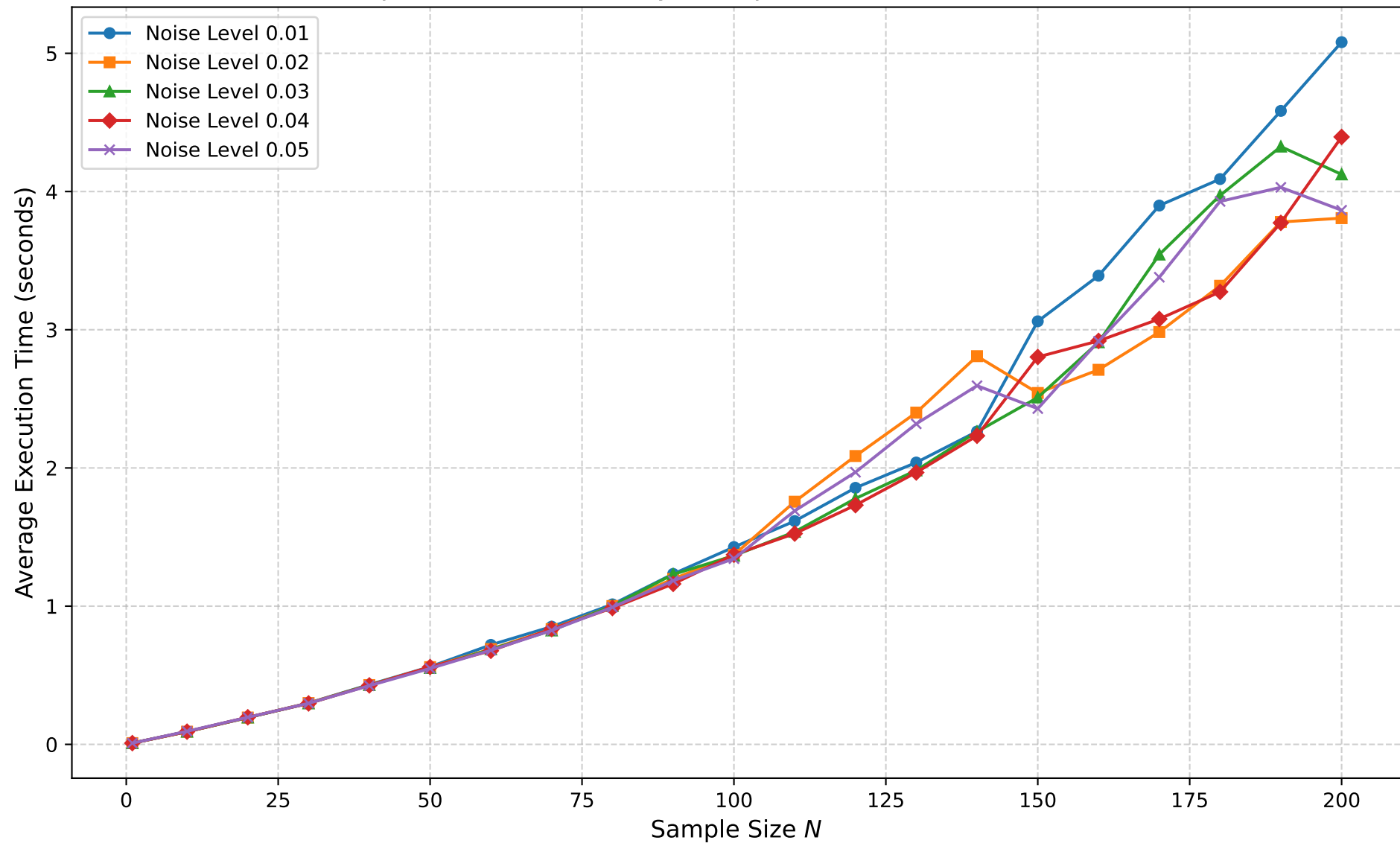
Computational Scalability: Sample Size N vs Execution Time
