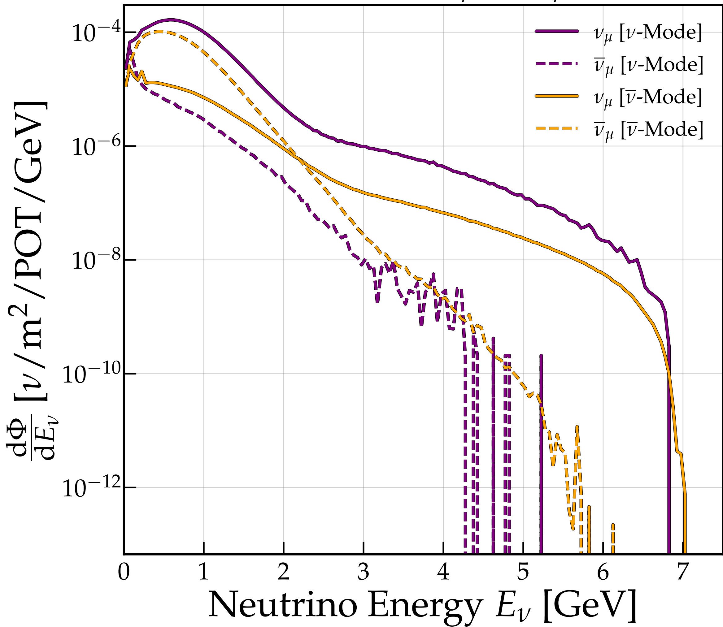
SBND Flux - \nu_\mu and \bar{\nu}_\mu
