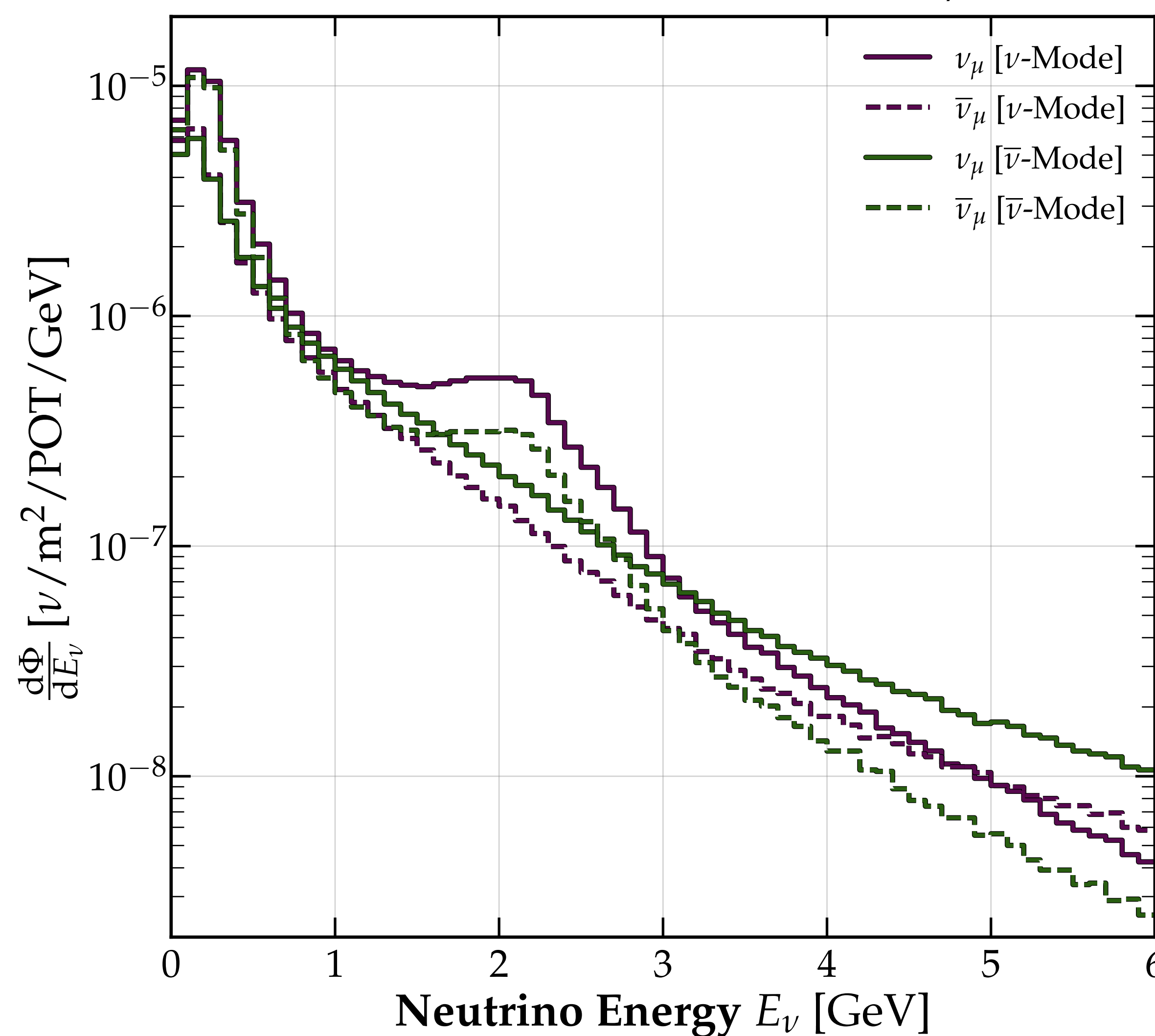
NuMI Off-axis Flux at ICARUS in \nu/\bar{\nu} Mode
