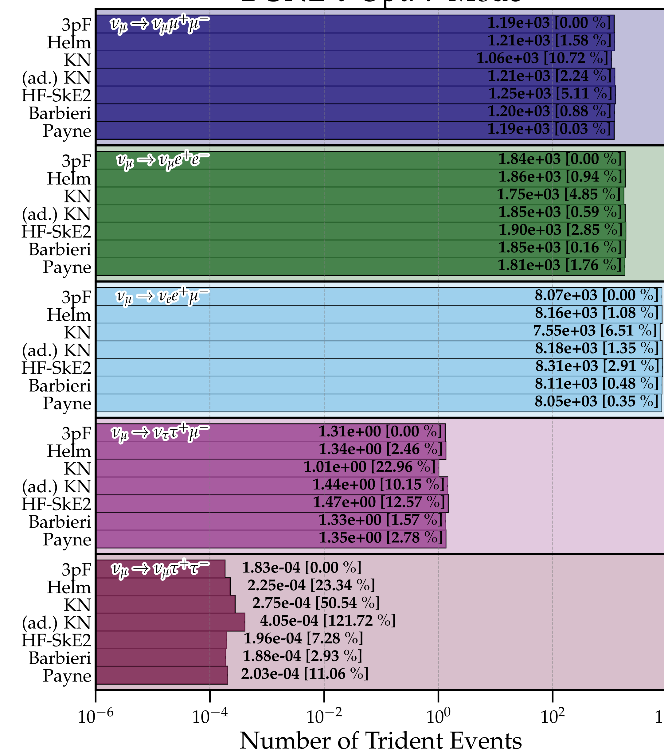
DUNE \tau -Opt. \nu -Mode
