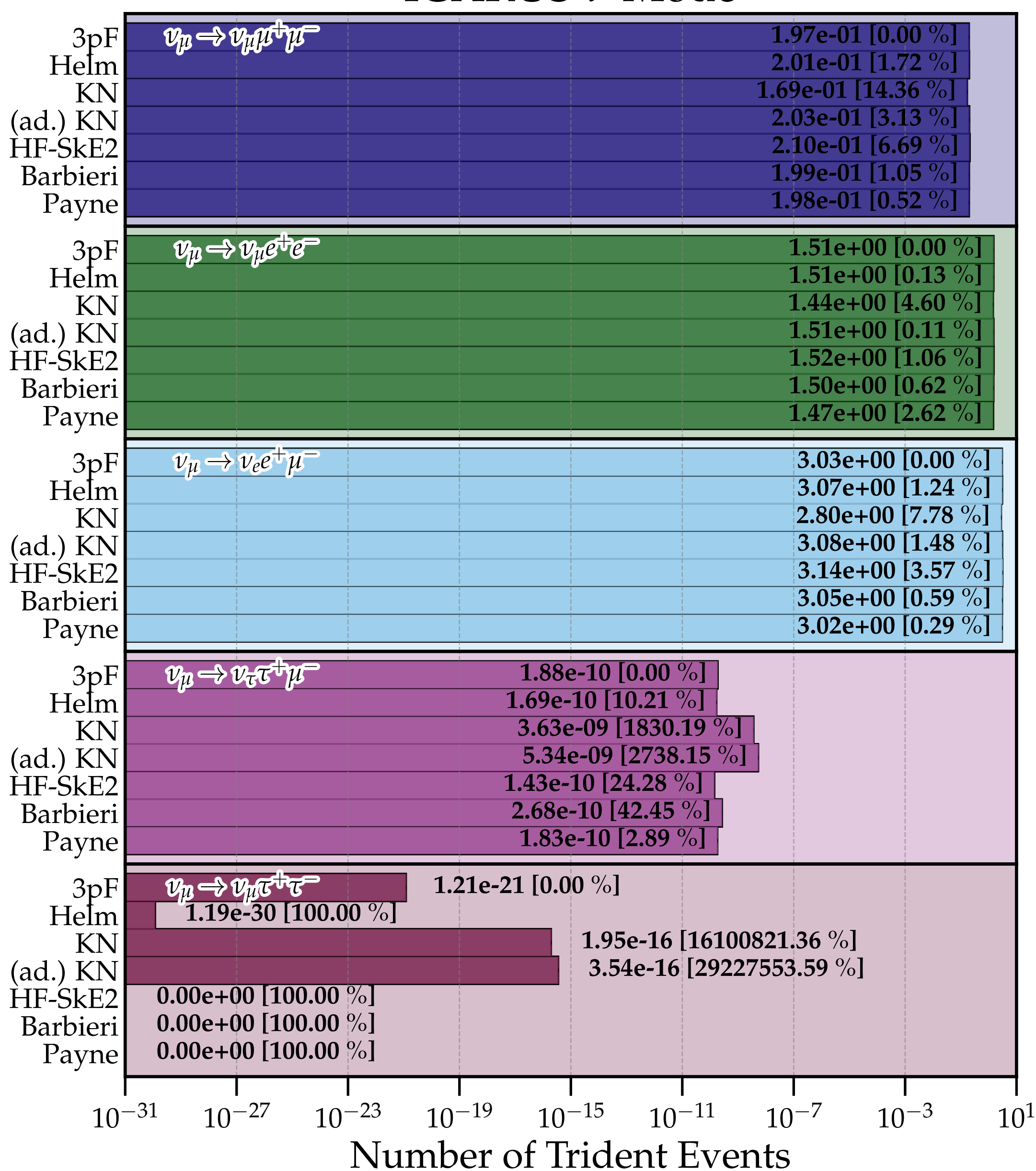
ICARUS \nu -Mode
