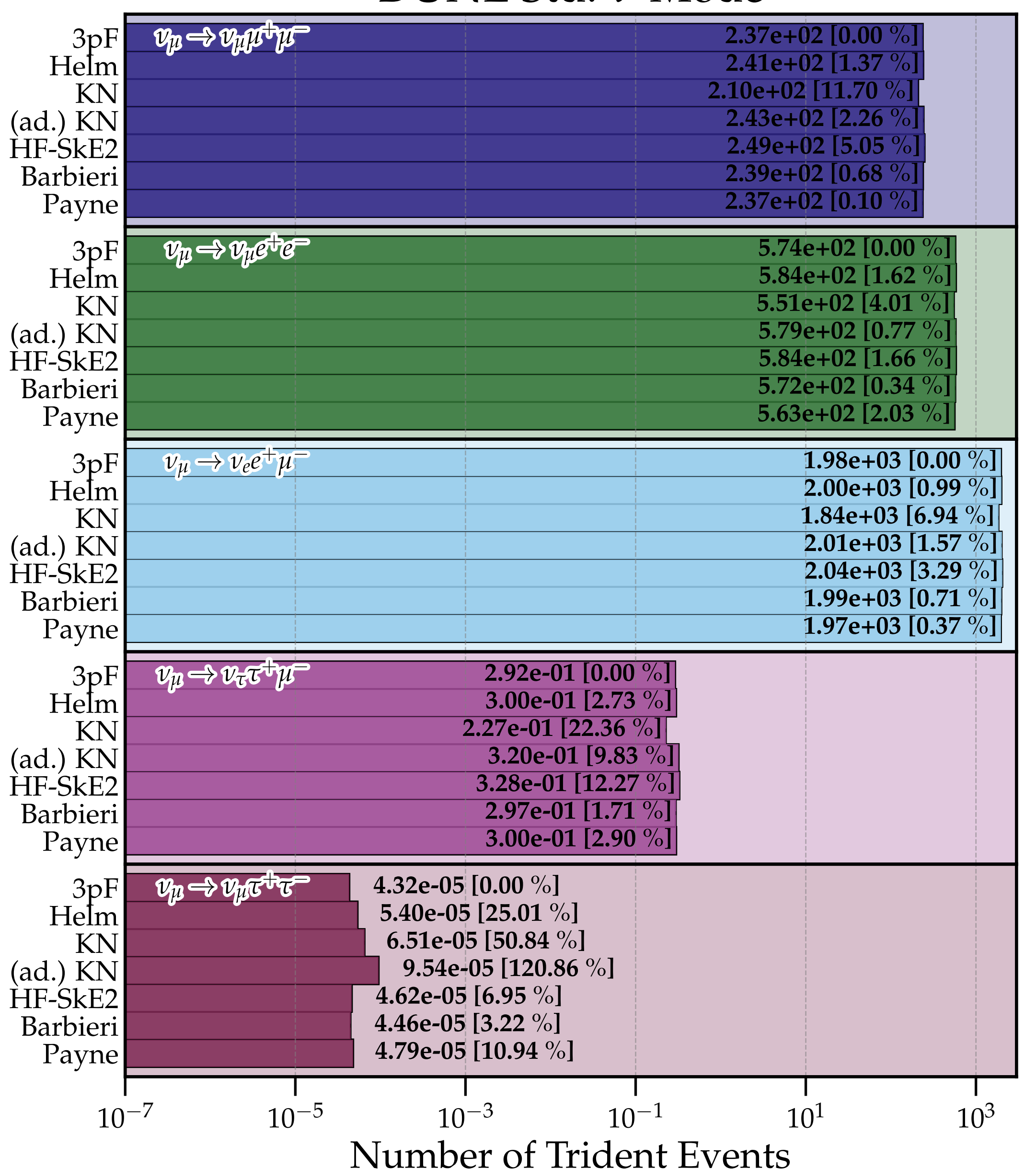
DUNE Std. \nu -Mode
