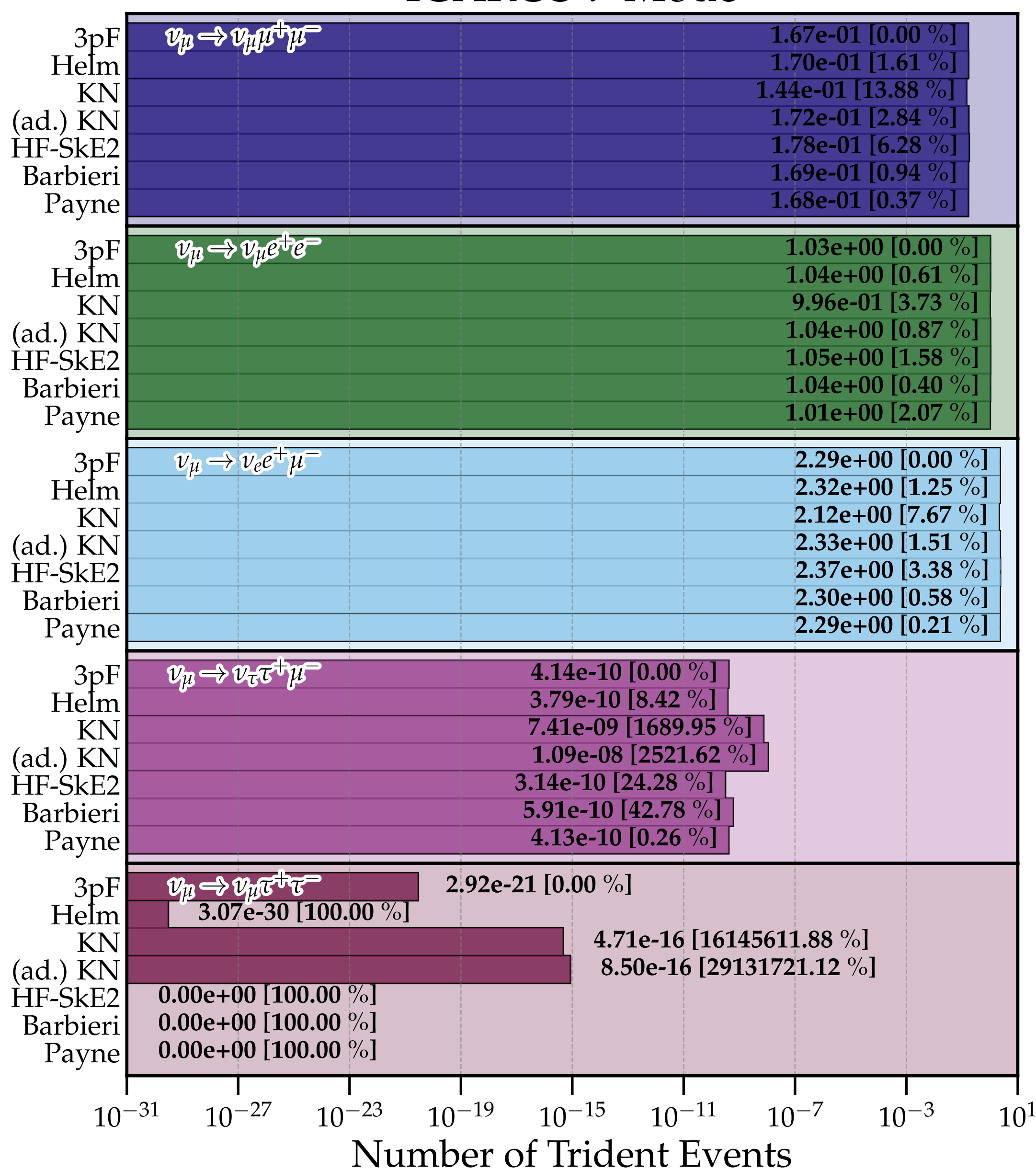
ICARUS \bar{\nu} -Mode
