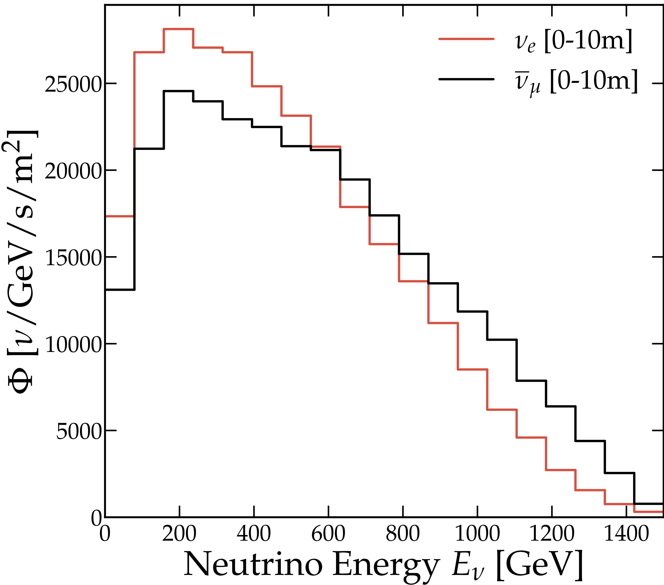
Forward Neutrino Flux MuC 3 TeV
