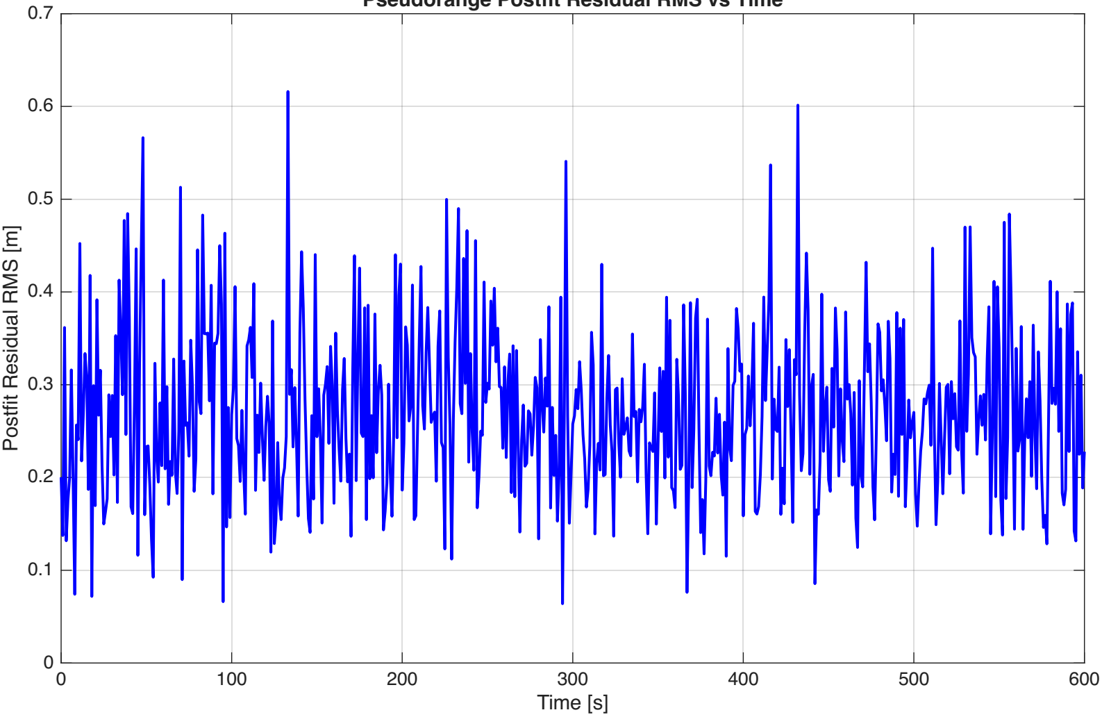
Pseudorange Postfit Residual RMS vs Time
