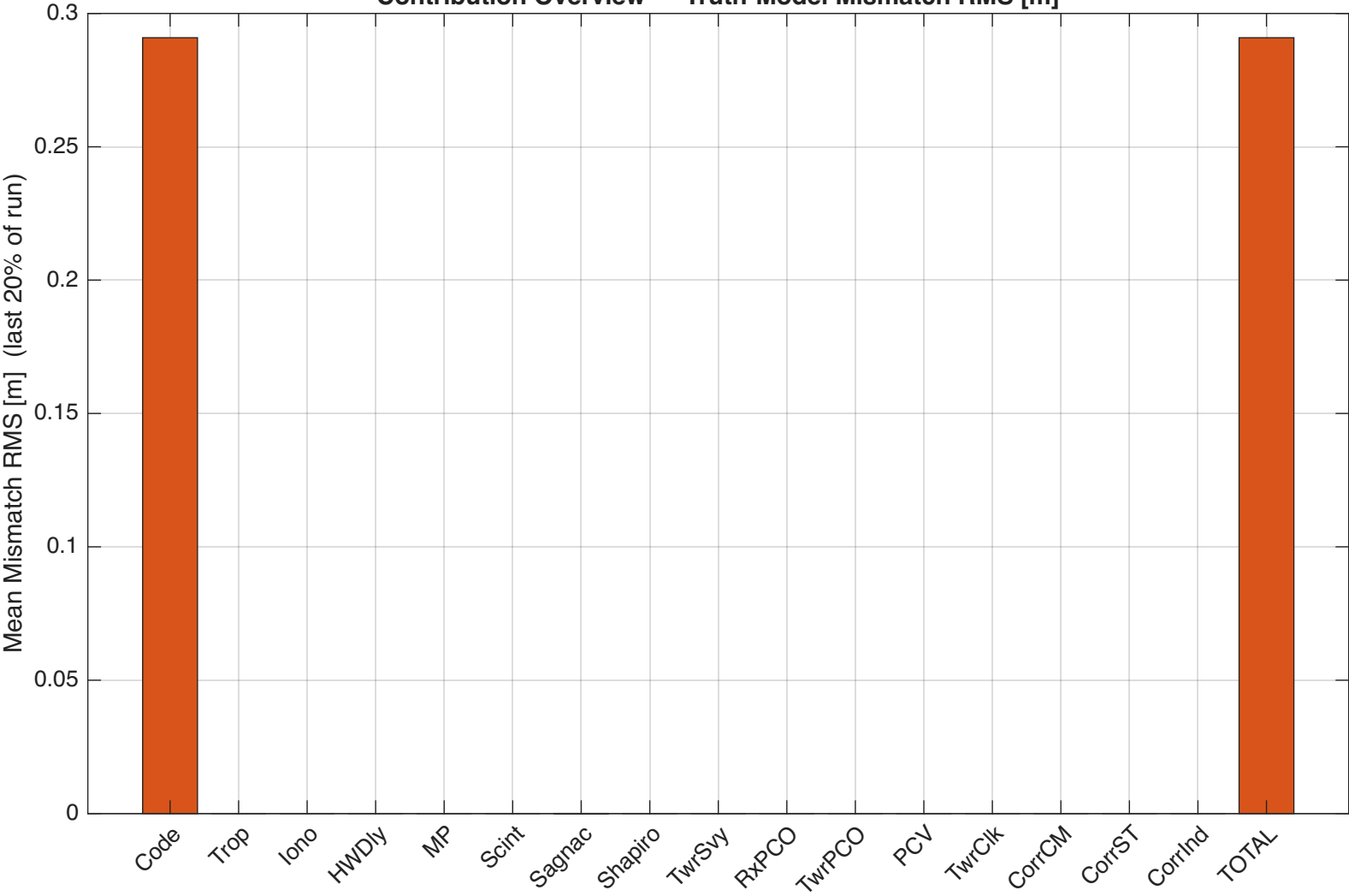
Contribution Overview — Truth-Model Mismatch RMS [m]
