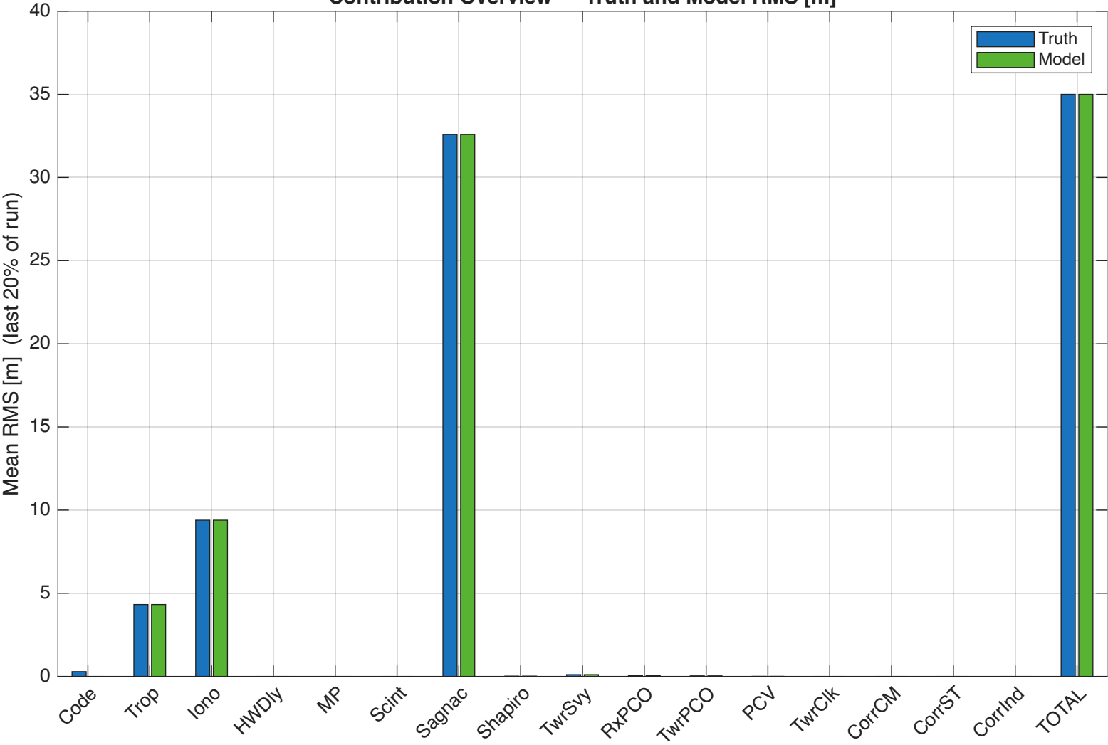
Contribution Overview — Truth and Model RMS [m]
