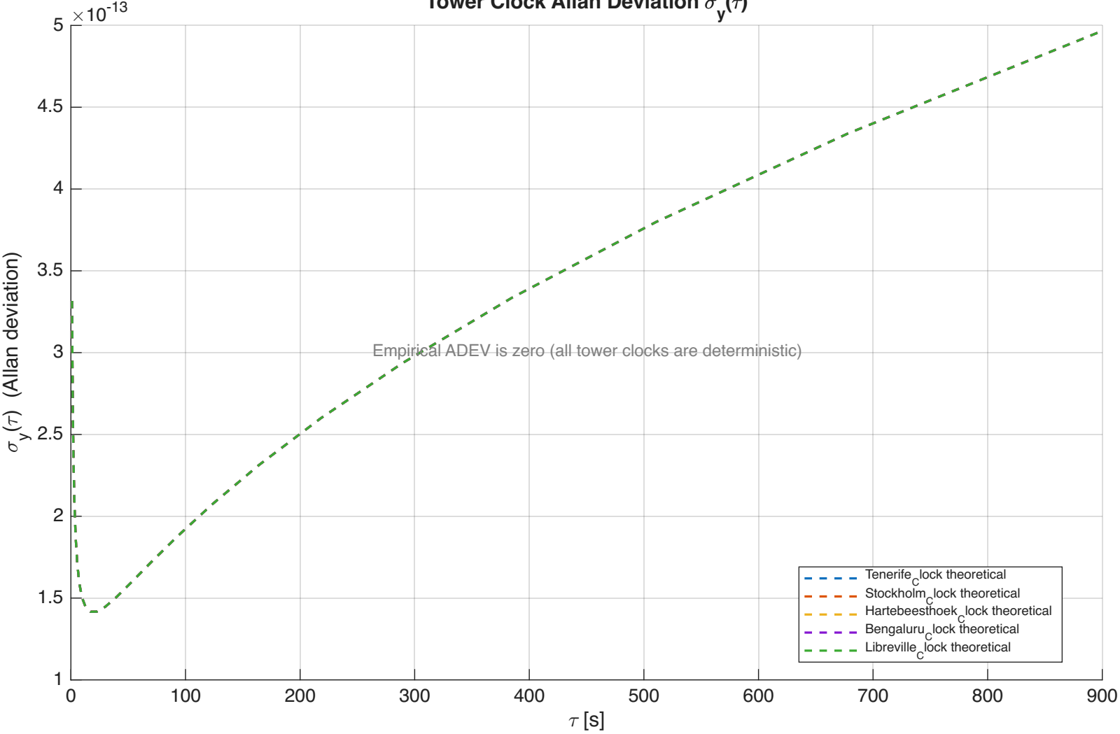
Tower Clock Allan Deviation \sigma_y(\tau)
