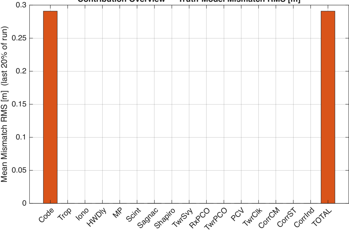
Contribution Overview — Truth-Model Mismatch RMS [m]
