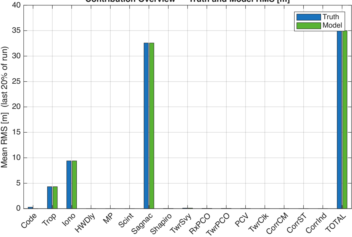
Contribution Overview — Truth and Model RMS [m]
