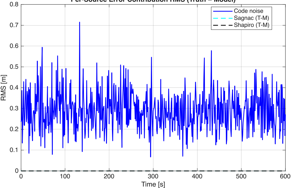
Per-Source Error Contribution RMS (Truth - Model)
