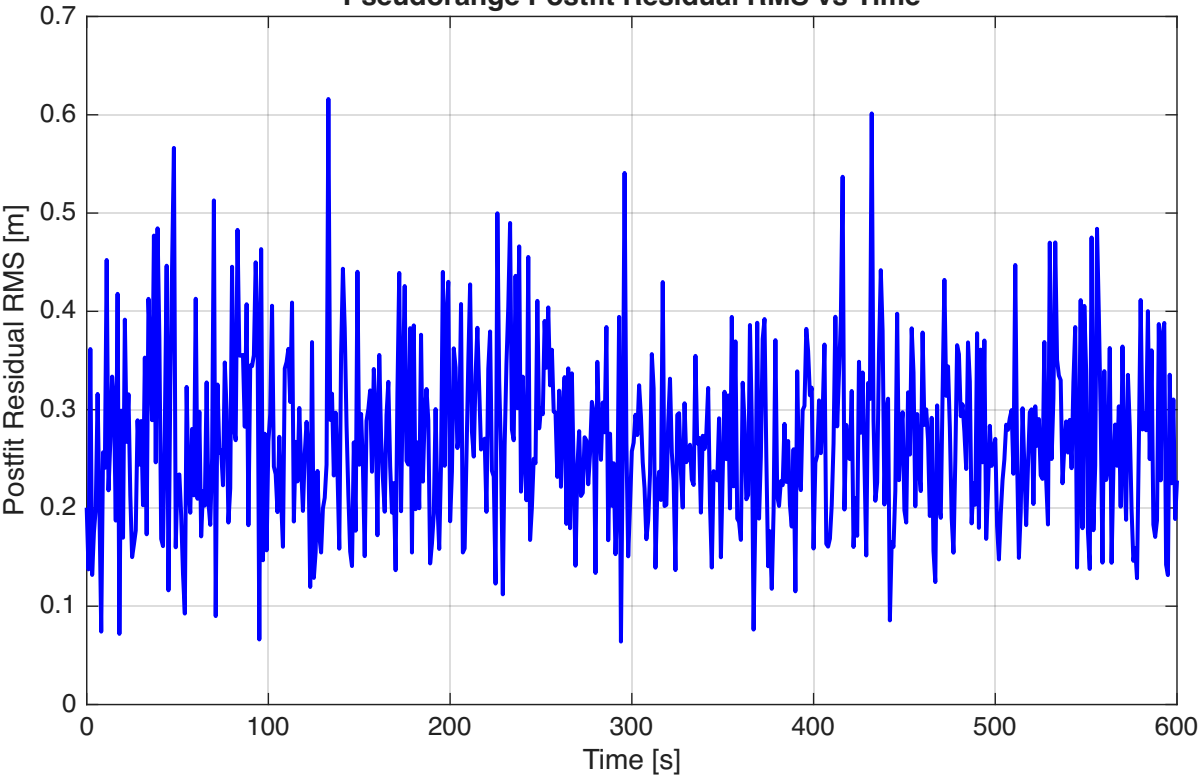
Pseudorange Postfit Residual RMS vs Time
