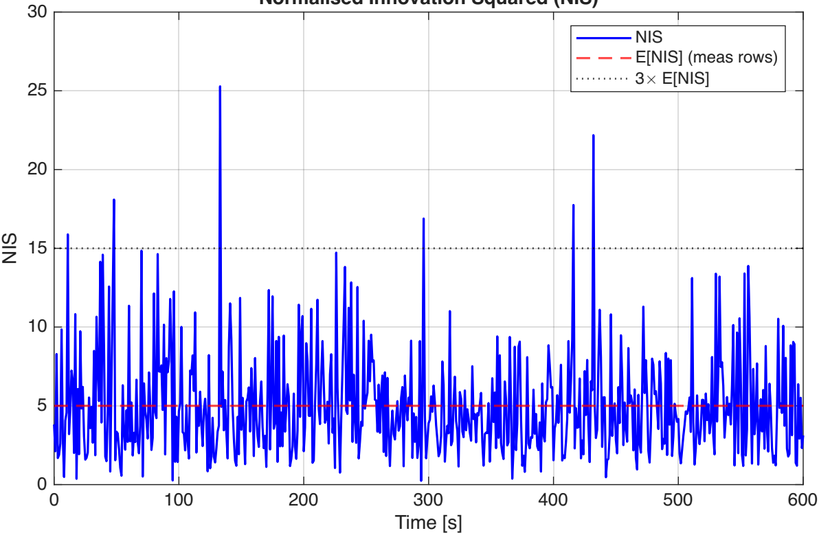
Normalised Innovation Squared (NIS)
