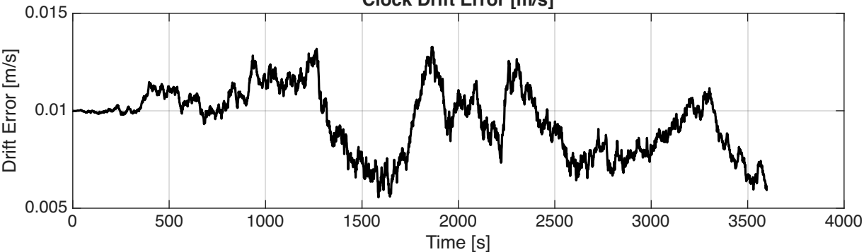
Clock Drift Error [m/s]
