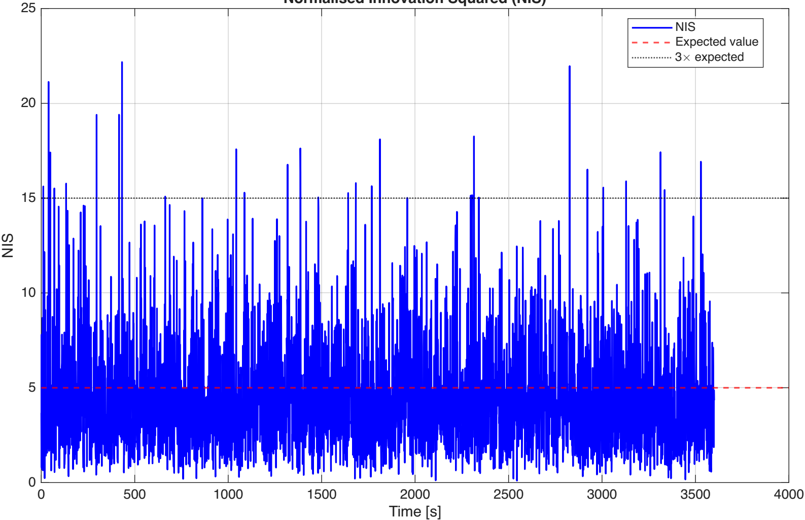
Normalised Innovation Squared (NIS)
