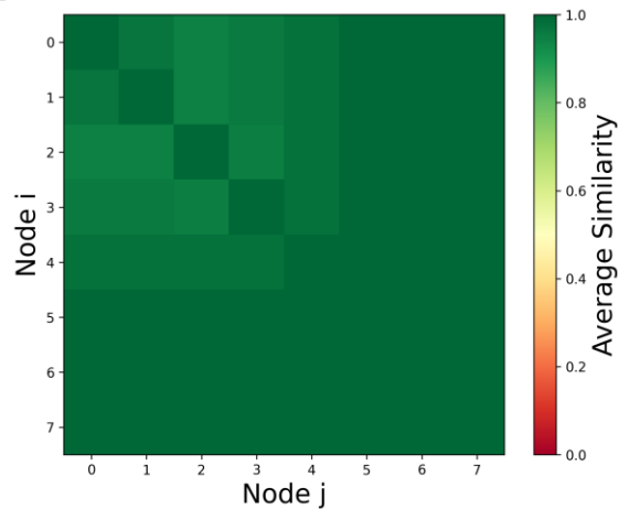
(a) Node-level similarity
