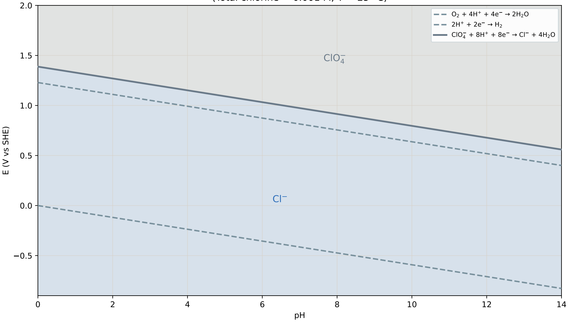
Chlorine Pourbaix Diagram (Total chlorine = 0.001 M; T = 25 °C)
