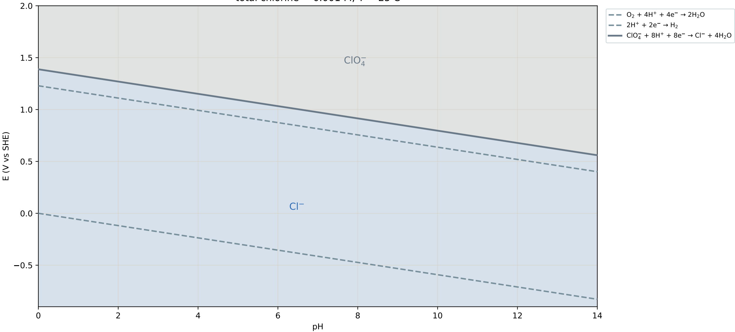
Teaching-scale chlorine Pourbaix diagram total chlorine = 0.001 M; T = 25 C
