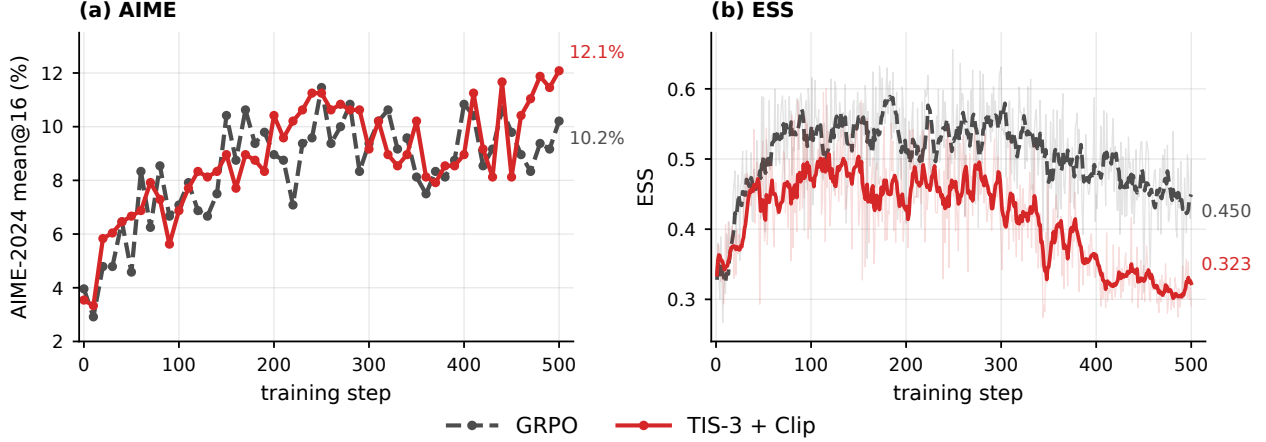
Figure 8: Qwen3-1.7B math RLVR at learning rate 10^{-6} . (a) AIME-2024 mean@16. (b) ESS, shown as raw observations (faint) and trailing seven-step means (thick). Dashed: GRPO. Solid: TIS-3 + Clip.
