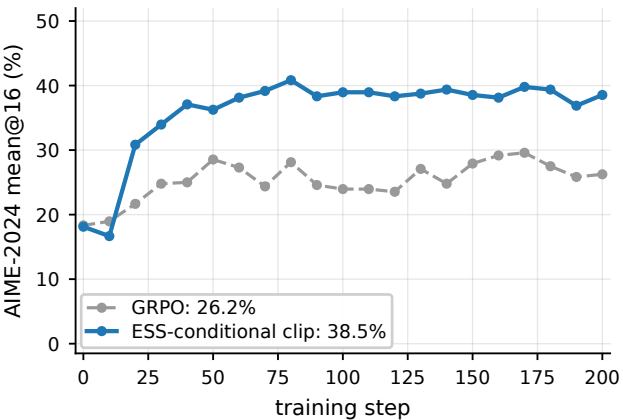
GRPO (band 0.2/0.2)
