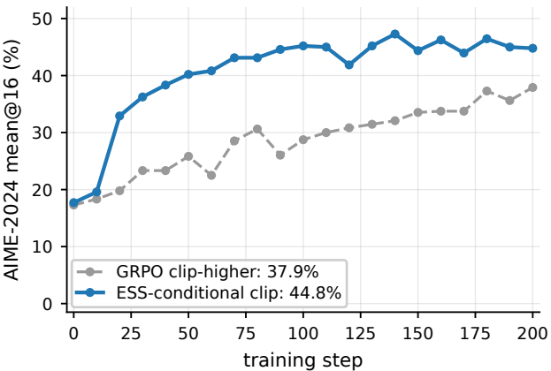
GRPO clip-higher (band 0.2/0.28)
