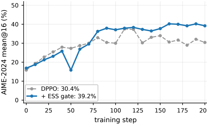
(c) DPPO
