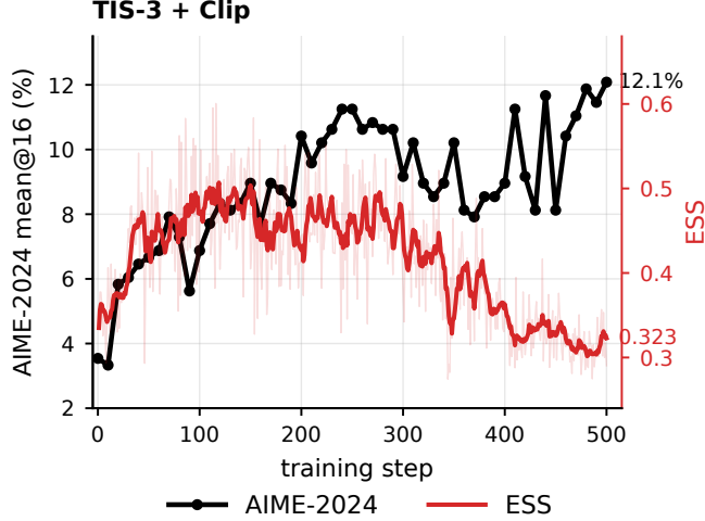
Figure 8: Qwen3-1.7B math RLVR with TIS-3 + Clip at learning rate 10^{-6} . Black, left axis: AIME-2024 mean@16. Red, right axis: ESS, shown as raw observations (faint) and a trailing seven-step mean (thick). End labels report the step-500 values.
