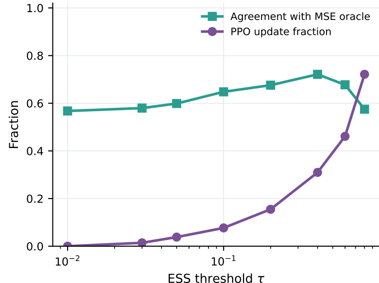
(c) What the heuristic approximates
