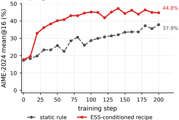
Clip-Higher
