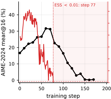
(a) TIS 3, no gate
