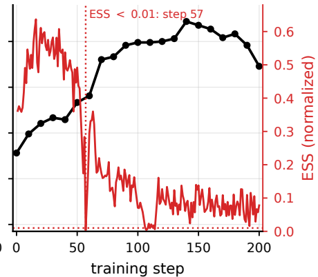
(c) GRPO, no clipping
