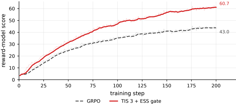
Open-ended RLHF
