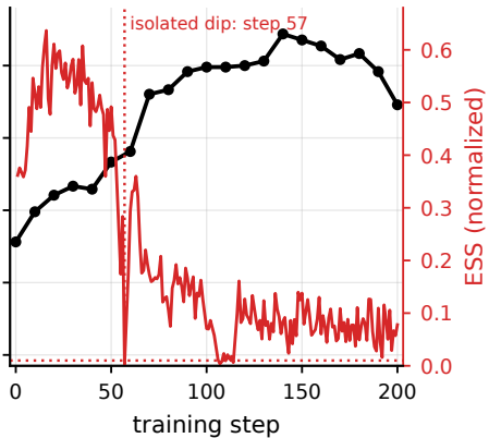
(c) GRPO, no clipping
