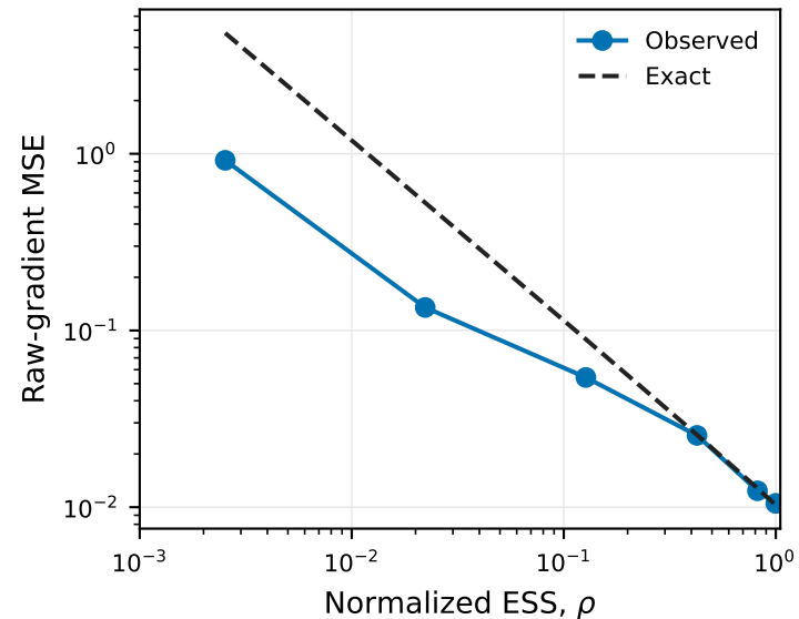
(a) ESS predicts gradient error
