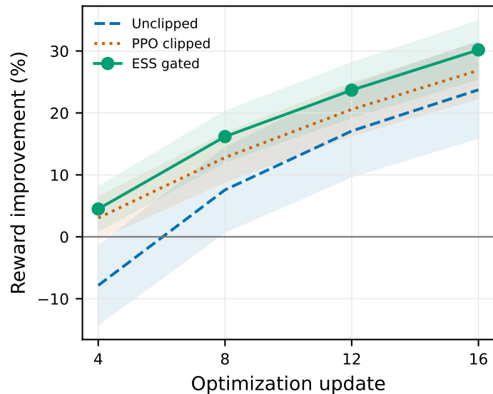
(c) ESS gating improves optimization
