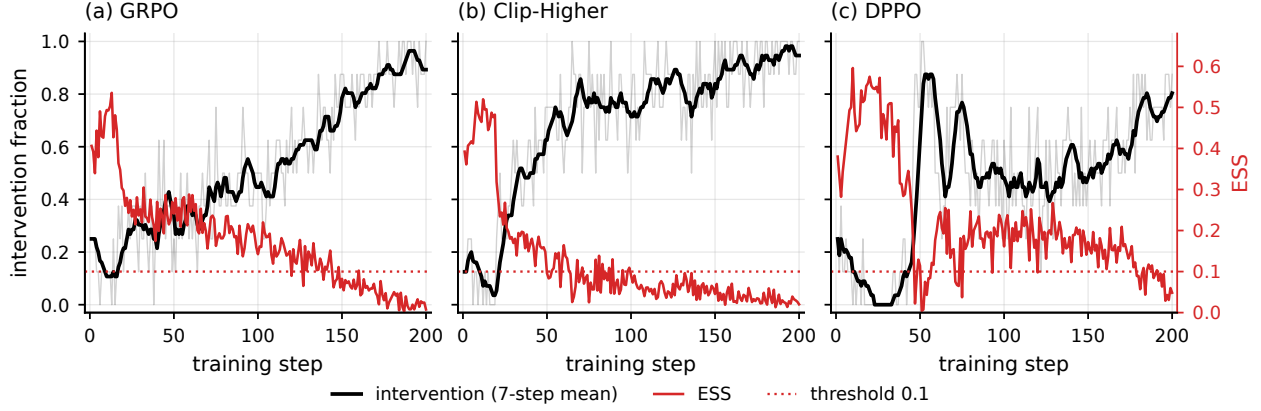
Figure 14: Realized ESS-conditioned intervention schedules. Each panel pairs the per-step intervention fraction (thin black) and its trailing seven-step mean (thick black) with ESS (red). GRPO and DPPO use raw ESS; Clip-Higher uses shaped ESS after the coefficient cap. The dotted line marks the threshold 0.1.
