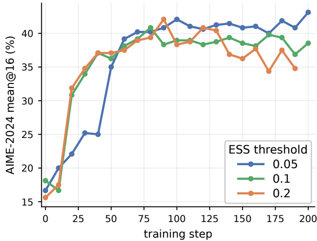
Figure 10: Sensitivity to the ESS threshold for TIS-3 with GRPO clipping on Qwen3-30B-A3B. Curves use \tau \in \{0.05, 0.1, 0.2\} ; clipping is activated when ESS falls below the corresponding threshold.
