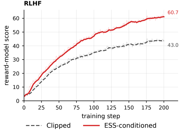
Figure 9: RLHF on Qwen3-4B-Instruct-2507 using Skywork-Reward-Llama-3.1-8B as the reward model. Thin curves show per-step scores and thick curves show trailing seven-step means. End labels report the step-200 observations.
