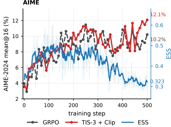
Figure 8: Qwen3-1.7B math RLVR at learning rate 10^{-6} . AIME-2024 mean@16 is shown for GRPO (dashed) and TIS-3 + Clip (solid). Blue: ESS for TIS-3 + Clip, shown as raw observations (faint) and a trailing seven-step mean (thick).
