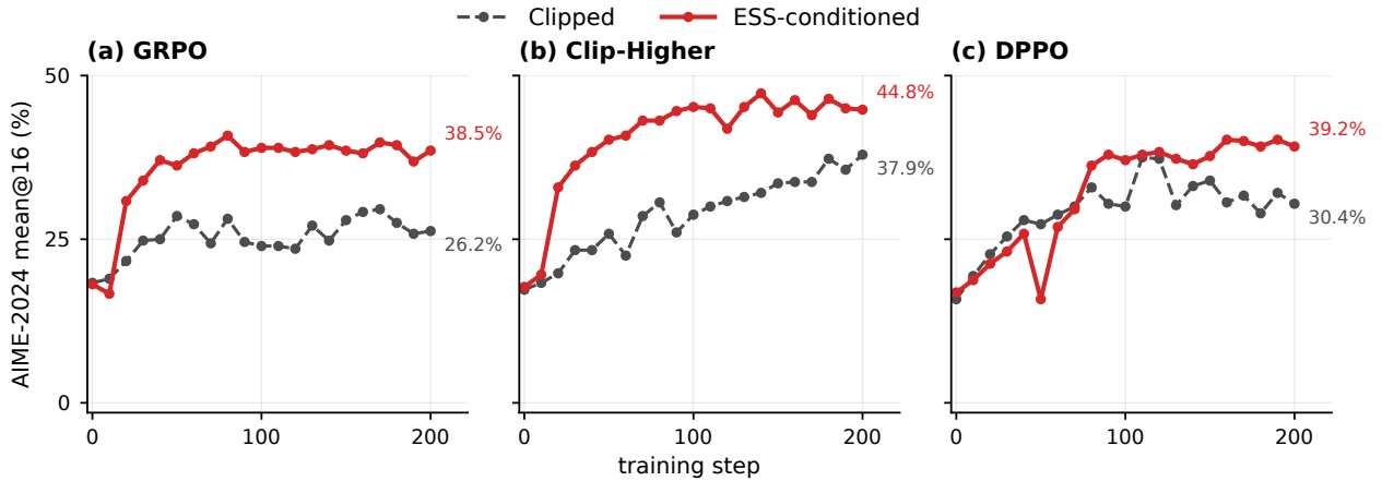
Figure 5: Qwen3-30B-A3B math RLVR over 200 policy updates. Dashed curves apply clipping throughout training. Solid curves begin with TIS-3 and switch to the corresponding clipped update when ESS falls below 0.1. (a) GRPO clipping. (b) Clip-Higher. (c) DPPO. End labels report the final observed AIME-2024 mean@16.
