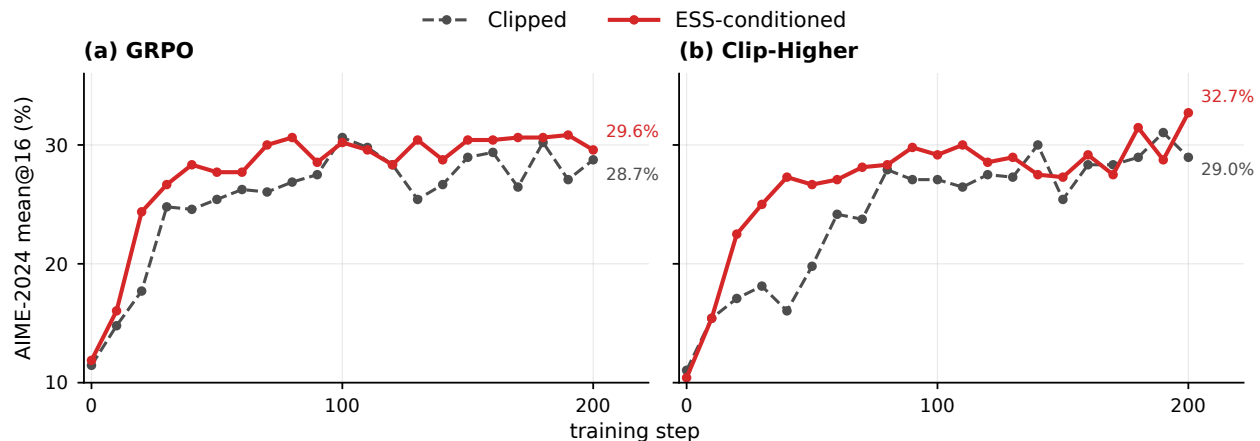
Figure 7: Qwen3-8B math RLVR over 200 policy updates. Dashed curves apply clipping throughout training, and solid curves use the ESS-conditioned counterpart. (a) GRPO. (b) Clip-Higher. End labels report the step-200 AIME-2024 mean@16.
