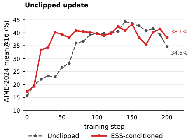
Figure 6: Qwen3-30B-A3B math RLVR with an unclipped update. Dashed: unclipped throughout. Solid: clipping below ESS 0.1. End labels report step-200 AIME-2024 mean@16.
