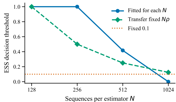
(b) The boundary moves with N
