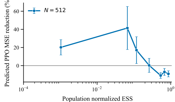
(a) Predicted crossover at informative N
