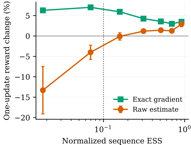
(b) Error changes update quality
