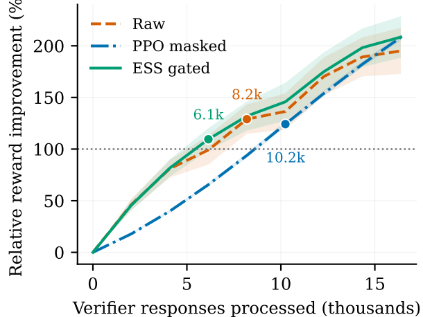
(c) ESS gate improves sample efficiency
