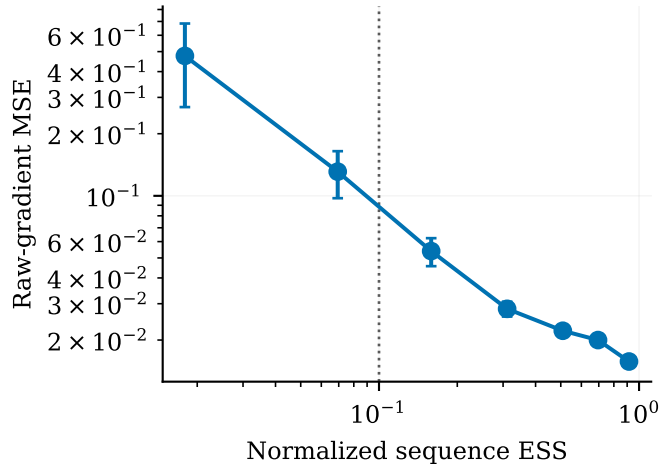
(a) ESS predicts gradient error
