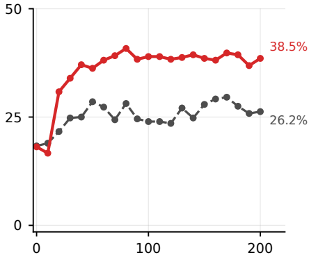
(a) GRPO
