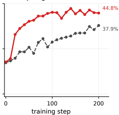
(b) Clip-Higher
