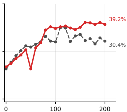
(c) DPPO
