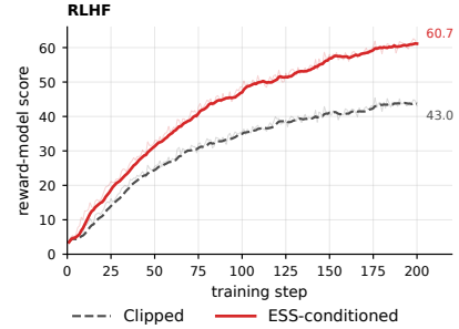
Figure 8: RLHF on Qwen3-4B-Instruct-2507. End labels report the step-200 observations.
