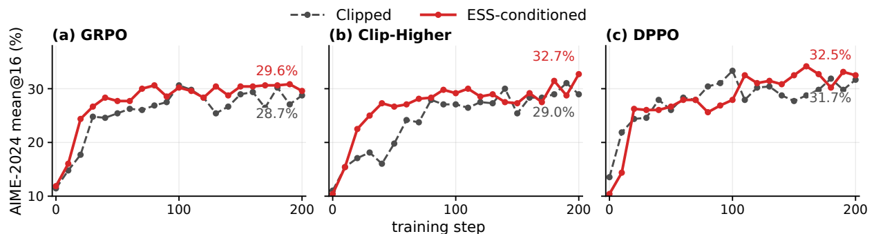
Figure 7: Qwen3-8B math RLVR over 200 policy updates. Dashed curves apply clipping throughout training, and solid curves use the ESS-conditioned counterpart. (a) GRPO. (b) Clip-Higher. (c) DPPO. End labels report the step-200 AIME-2024 mean@16.
