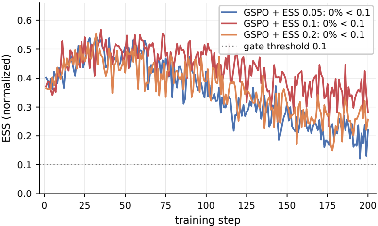
GSPO ablation — sequence ESS
