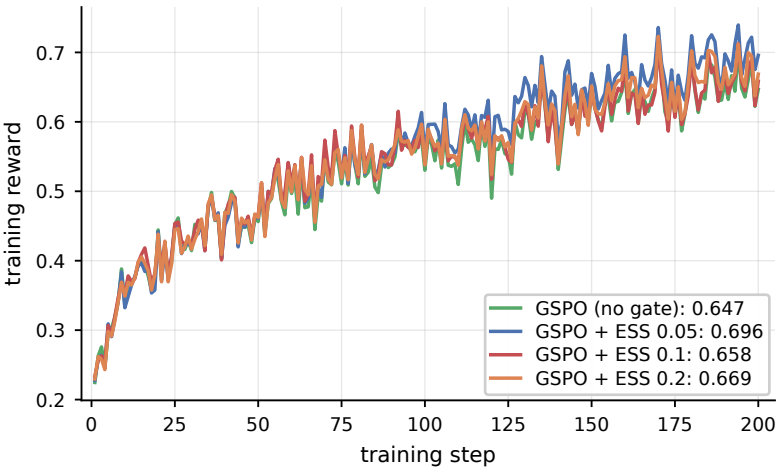
GSPO ablation — reward
