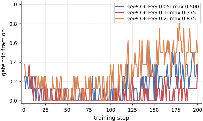
GSPO ablation — gate trip
