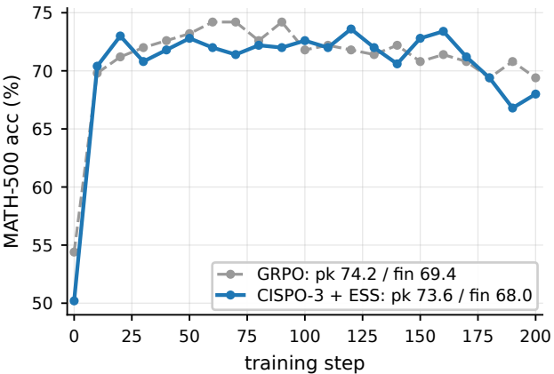
Qwen2.5-7B: MATH-500
