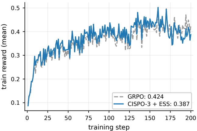
(a) training reward
