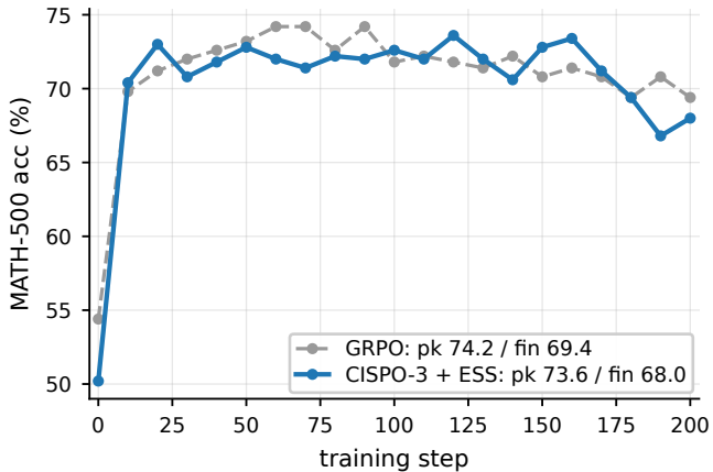
(b) MATH-500 accuracy
