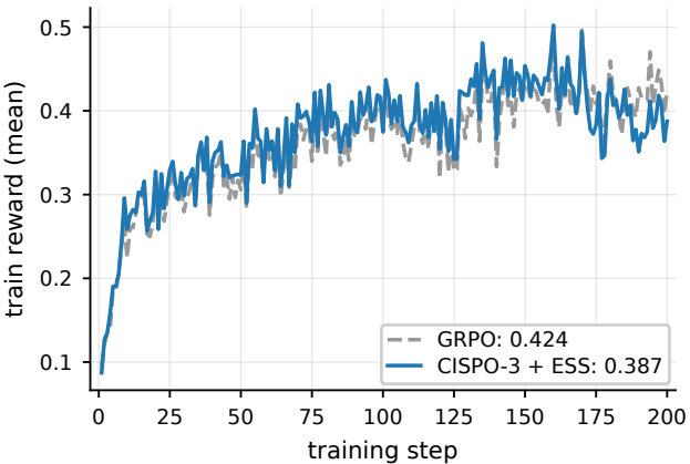
Qwen2.5-7B: training reward
