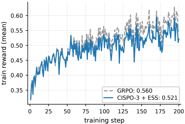
R1-1.5B: training reward
