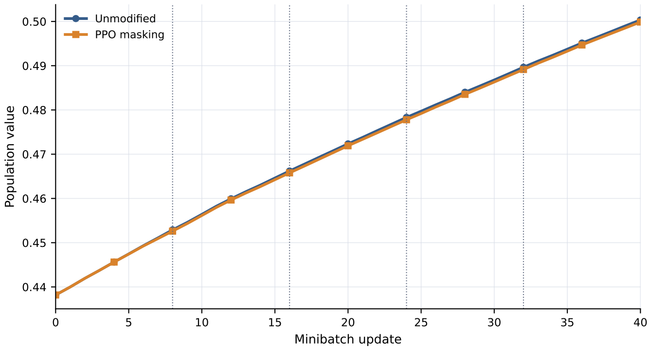
Certified-step learning across all 40 updates
