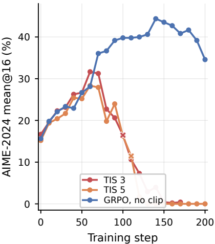
(a) Validation performance
