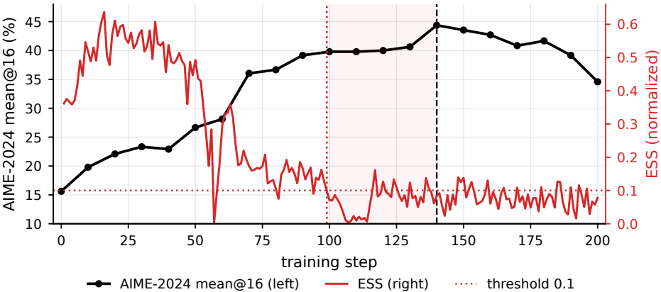
GRPO, no clipping
