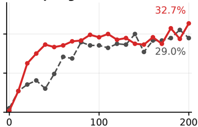
(b) Clip-Higher
