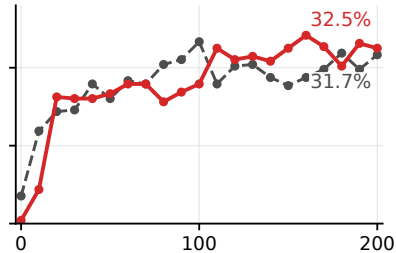
(c) DPPO
