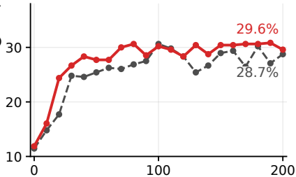
(a) GRPO
