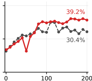
(c) DPPO
