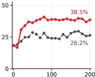
(a) GRPO
