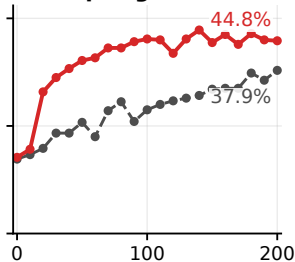
(b) Clip-Higher
