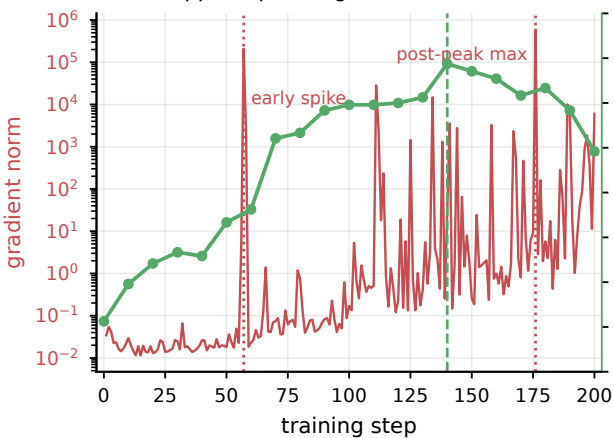
(c) Unclipped update: gradient norm
