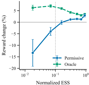
(b) One-step policy improvement
