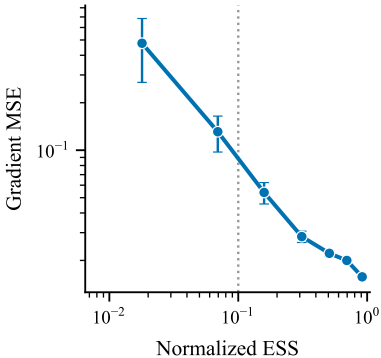
(a) Gradient estimation error
