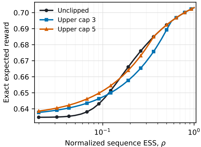
(b) One-step policy value
