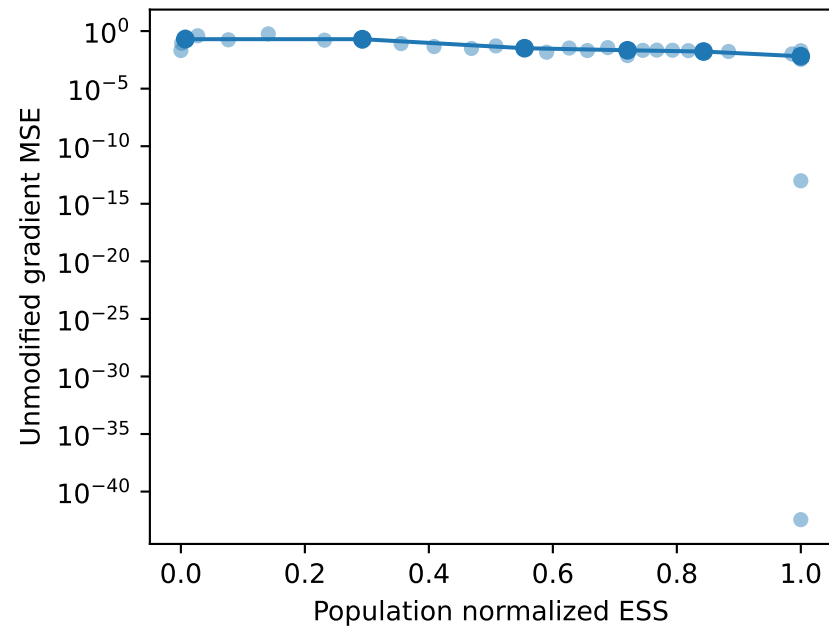
ESS and estimator error
