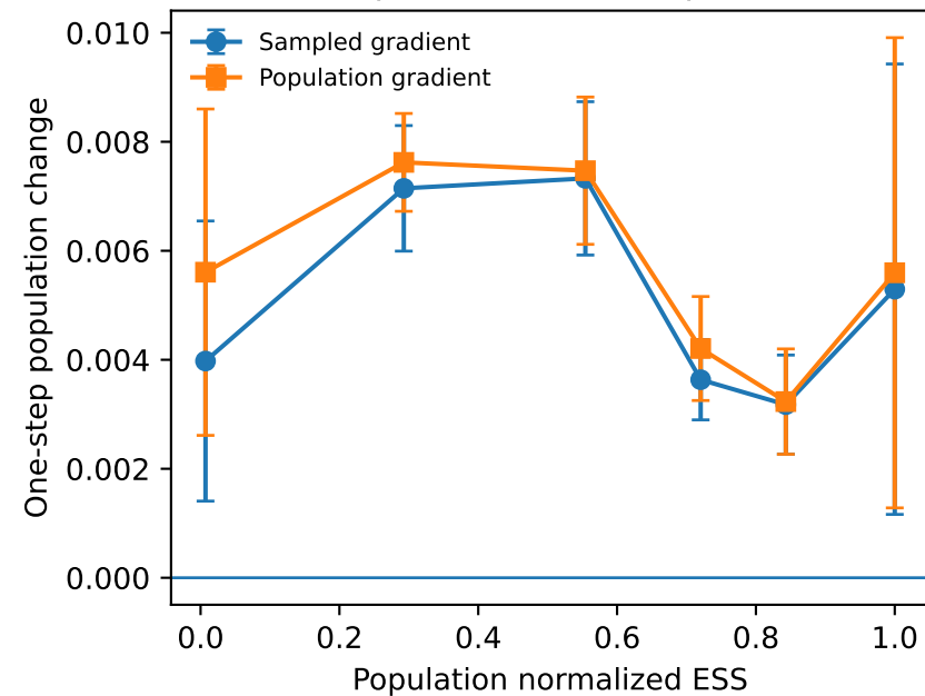
Sampled and oracle updates
